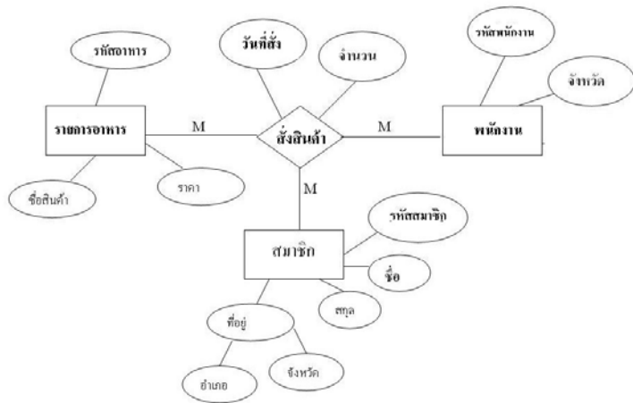
ER-diagram
